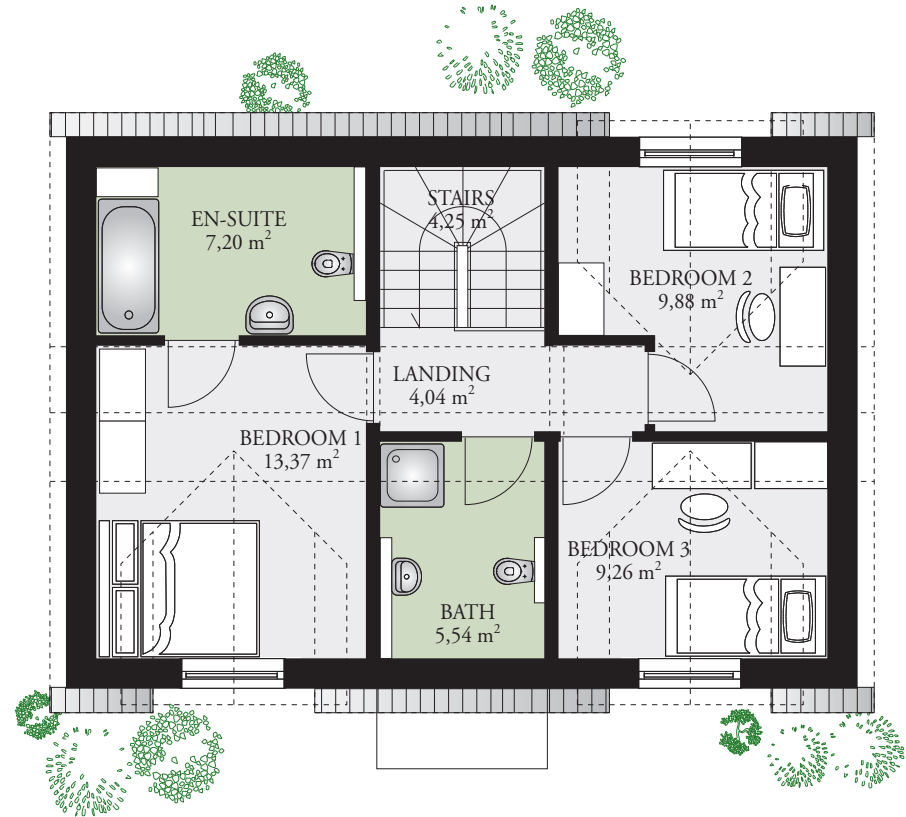
FIRST FLOOR AREA 56,93 m 2 (613 sq ft)
