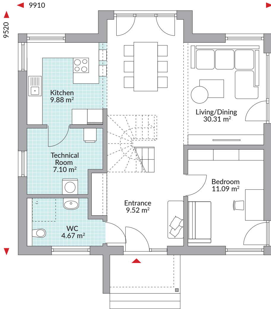
GROUND FLOOR AREA 75.80 m 2 (816 sq.ft.)
