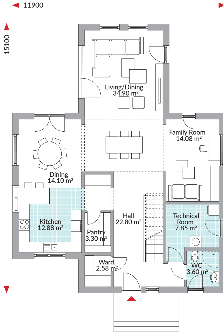
GROUND FLOOR AREA 120.41 m 2 (1,296 sq.ft.)
