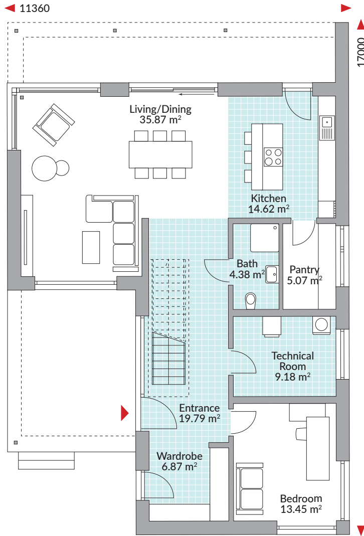
GROUND FLOOR AREA 114.00 m 2 (1,227 sq.ft.)
