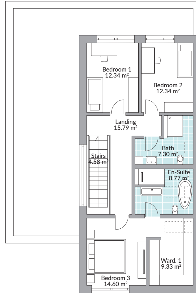
FIRST FLOOR AREA 86.85 m 2 (935 sq.ft.)
