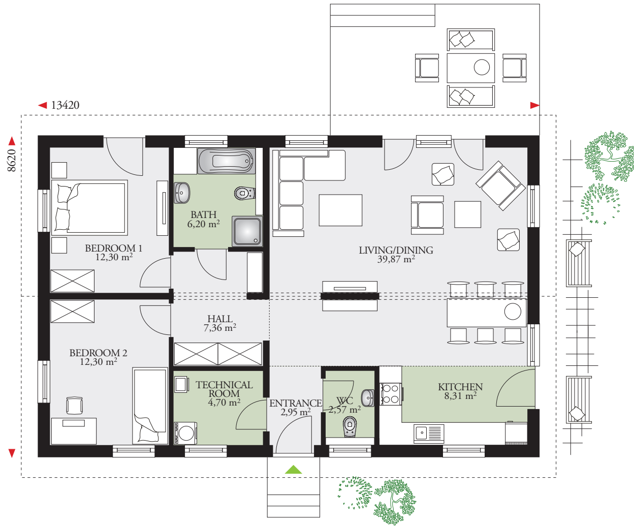
GROUND FLOOR 100,95 m 2 (1087 sq ft)
